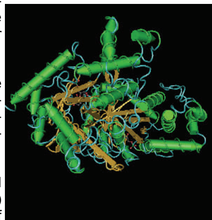
Crystal Structure Of Plasmodium Falciparum Orotidine 5'-Phosphate Decarboxylase Covalently Modified By 6-Iodo-Ump
